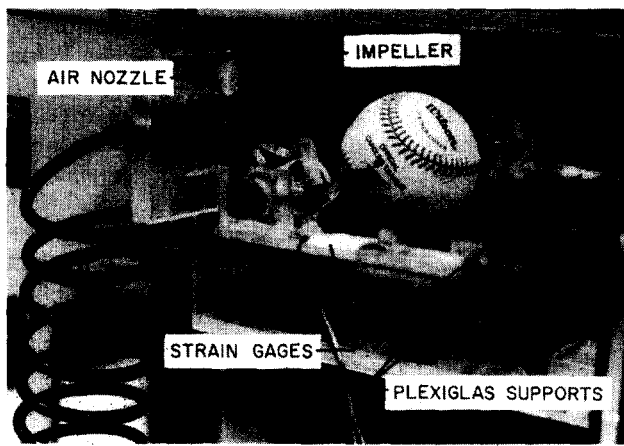
Fig. 3. The experimental device.
