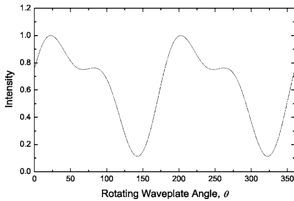
Fig. 4. Intensity plot for Eq. (23) for the continuous rotation of the quarter-waveplate through 360°, showing two identical waveforms; the period of a single waveform is 180° and repeats over 180° intervals.
